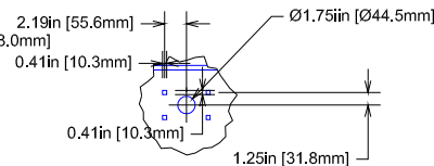
DETAIL B Fault Indicators
